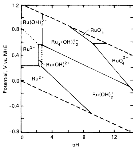
Figure 1. Potential–pH diagram for Ru–H 2 O at 298 K and a total Ru concentration of 10^{-6} mol L -1 . This calculation is for the aqueous phase only, and no precipitates have been allowed to form. Dashed lines are for the water stability field, and dotted lines indicate regions that are fairly uncertain due to the uncertainty in \psi . Boundary lines between species indicate where concentrations are equal. Redrawn from Isherwood. 480
